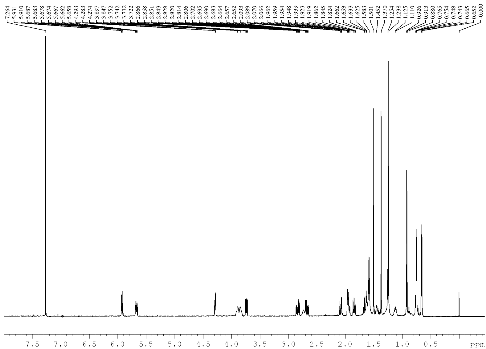
Figure 1. ^1\text{H} NMR (500 MHz) of trichoharzianol in \text{CDCl}_3 .
