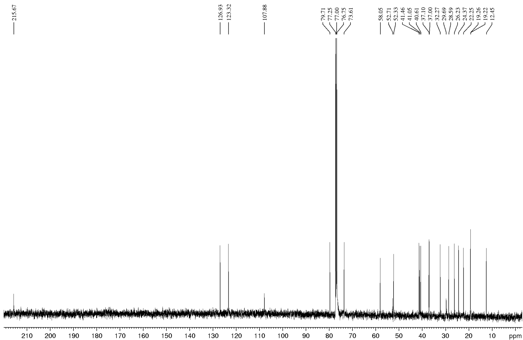
Figure 2. 13 C NMR (125 MHz) of trichoharzianol in CDCl 3 .
