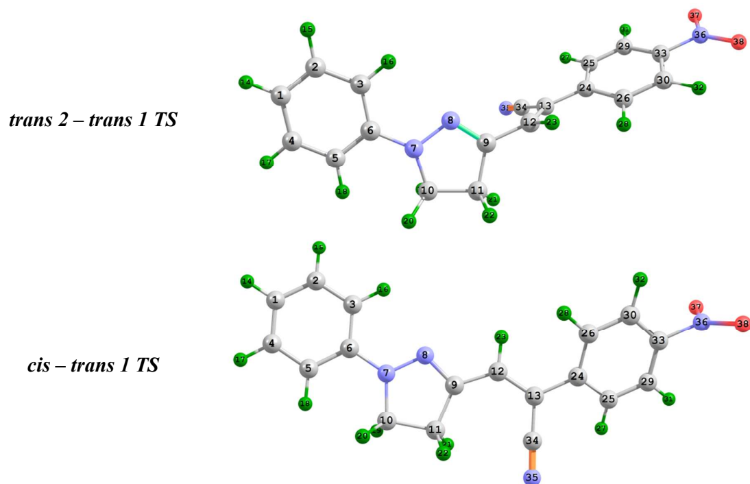
Figure S1. Optimized molecular structures of transition states between trans 2 - trans 1 and cis - trans 1 conformers of PY-oCNNO 2 ; DFT/B3LYP/6-311++G(d,p). Atom colors: C – gray, H – green, N – blue, O - red.
