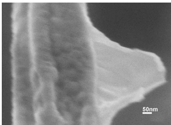
Figure S2. High magnification SEM image of nanofibers after peeled off using ultrasonication for 5s.
