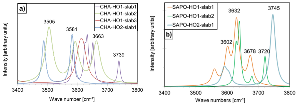
Figure S2 Computed IR spectra of the vacuum slabs of a) H-CHA and b) H-SAPO, from which the matching models in Fig. 8 could be reconstructed by adding them together after adequate peak intensity adjustments. Here the spectra are shown at common scale for better visibility.
