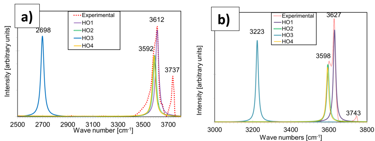
Figure S1 Experimental TR (copied from Fig. 1) and computed OH spectra of a) H-CHA and b) H-SAPO-34 with all four HOn positions where n = the oxygen position numbers in Fig 2.
