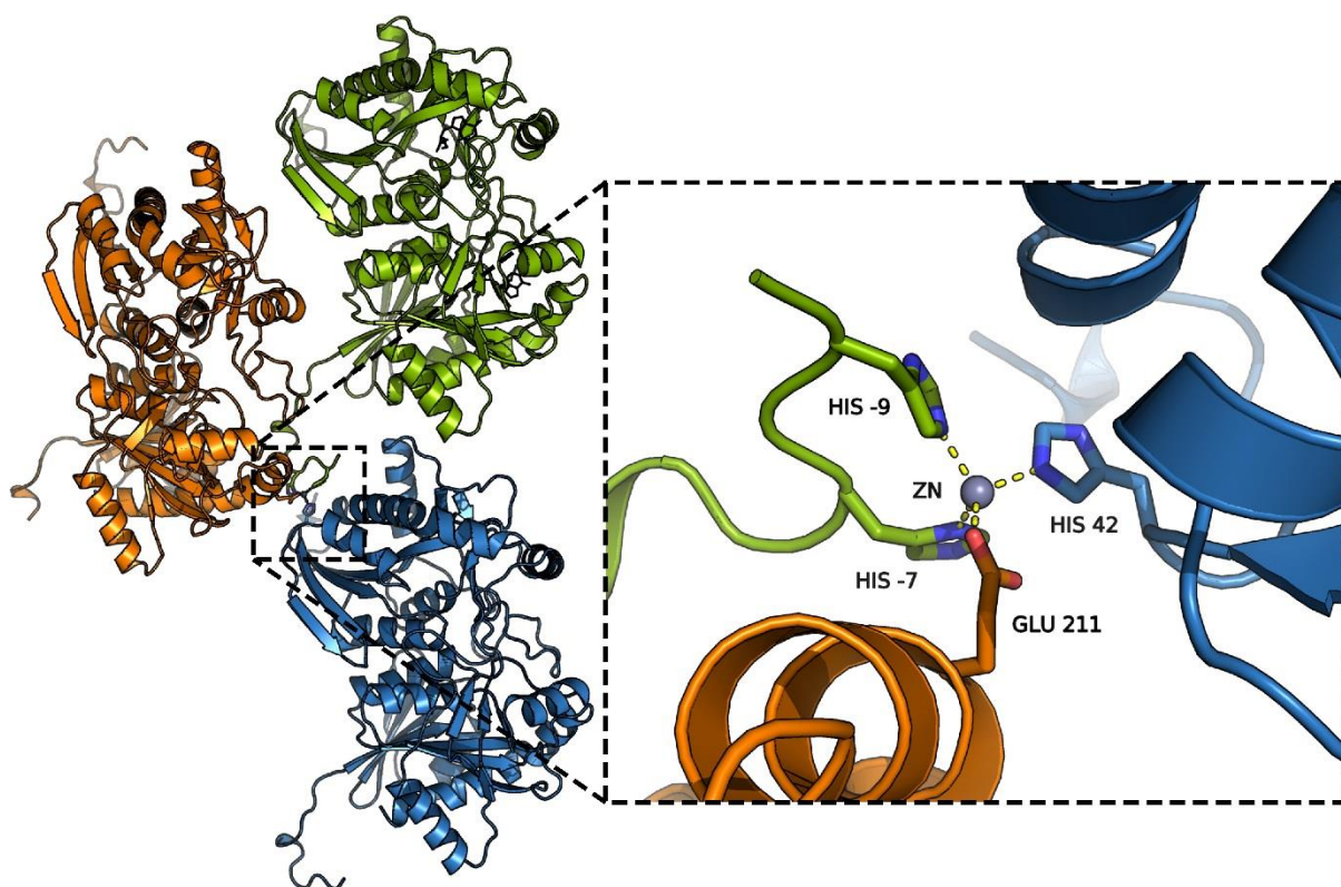
Figure. Three Hp MTAN dimers with 54 bound, illustrating the tetrahedral zinc coordination complex formed by fusion tag histidine residues (His -7 and His -9) and main chain residues (His 42 and Glu 211) from neighboring dimers.
