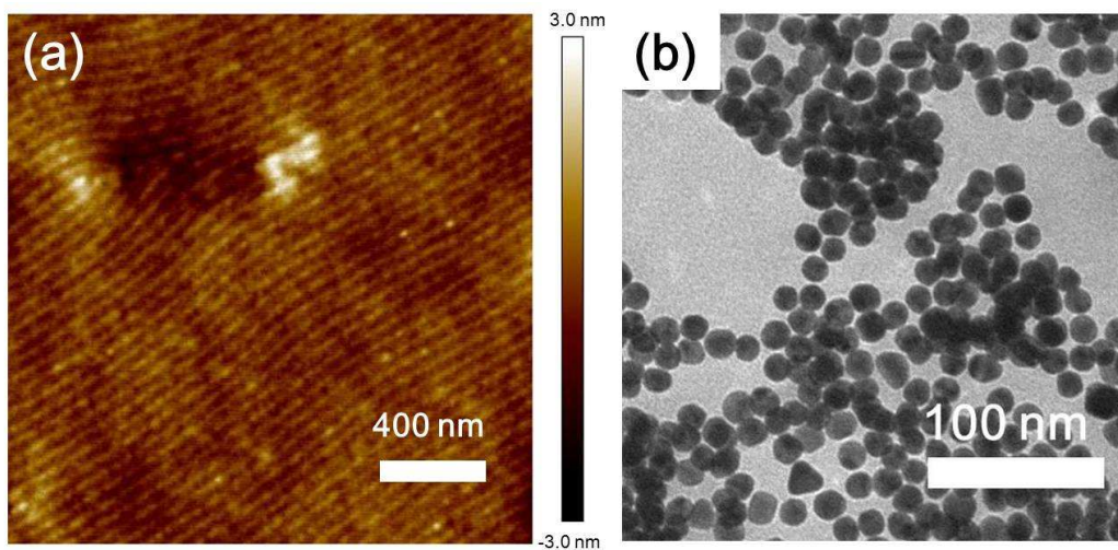
Figure S1. (a) AFM height image of PS- b -P2VP (62k-26k) cylinder-forming block copolymer template. (b) TEM image of as-synthesized gold nanoparticles.
