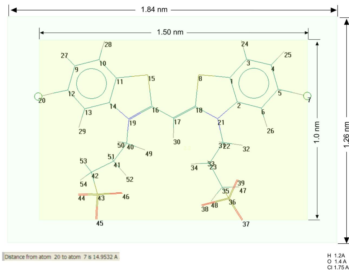
Figure S1. The dimensions of the TC molecule with mostly extended sulfopropyl chains obtained on the base of the Chem Draw modeling (inner yellow rectangle). The outer light yellow rectangle additionally includes van-der-Waals radii of outer Cl, O, and H atoms.
