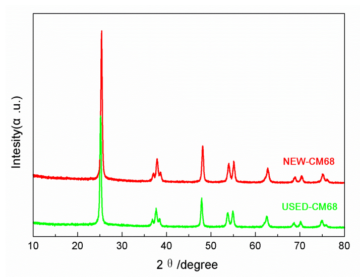
S_Figure 2. XRD patterns of fresh and used CM68 catalysts.
