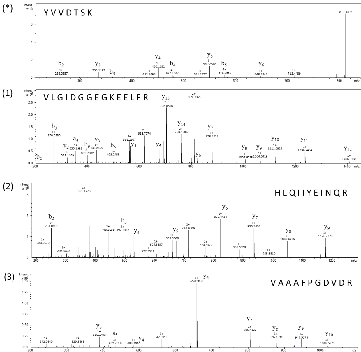
Figure S-1. Annotated MS/MS spectra of four peptides measured with the PASEF method as shown in Figure 4.
