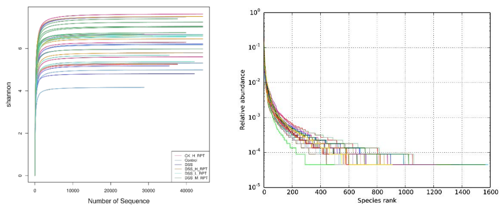
Figure. S1 Shannon curves (a), rank abundance (b).
