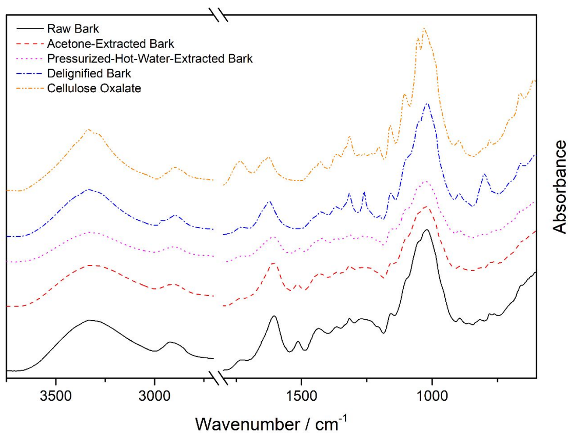
Figure S1. ATR-FTIR spectra of all samples after each processing step.
