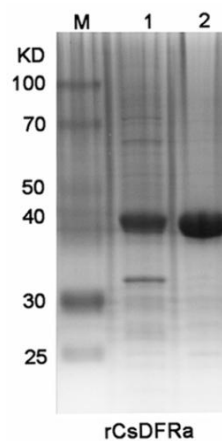
Figure S2 SDS-PAGE gel of rCsDFRa protein. M indicate the marker, the number 1 indicated the protein before purification and number 2 indicate the purified protein.
