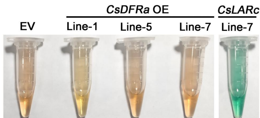
Figure S3 DMACA staining of the extracts from CsDFRa transgenic tobacco flowers and control flowers. Note, CsLARc transgenic tobacco was served as a positive control. EV represent empty vector control.
