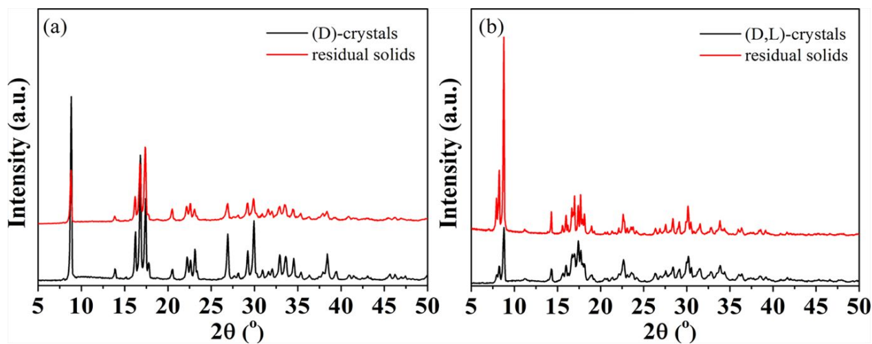
Figure S1. PXRD patterns of the raw crystals and the residual solids after solid-liquid equilibrium in the mixture solvent of (D)-penicillamine (a) and (D,L)-penicillamine (b).
