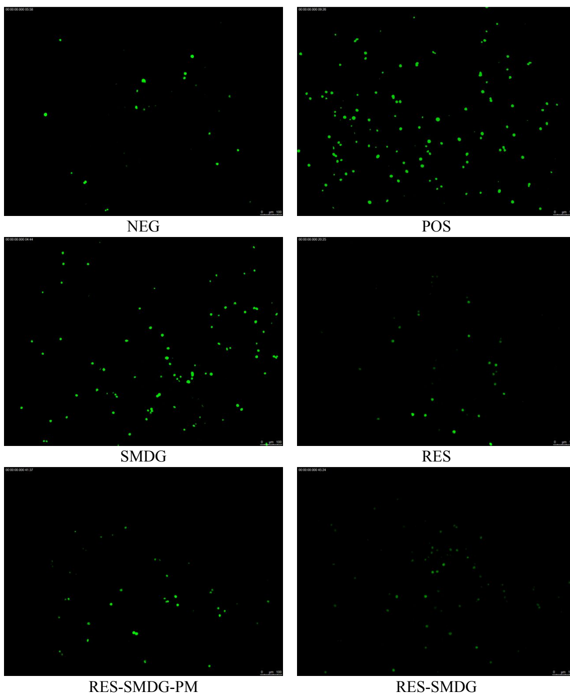
Figure S1 ROS levels detected by dichlorodihydrofluorescein diacetate (DCFH-DA) assay
