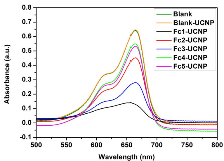
Figure S7. UV-Vis absorption spectra of removal of MB.
