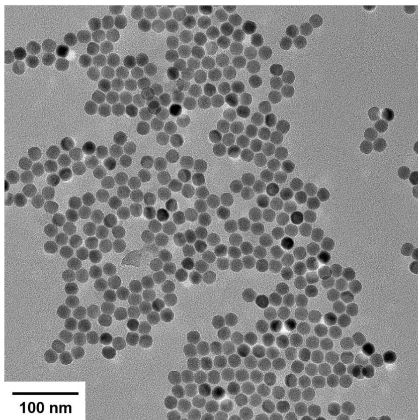
Figure S2. TEM images of OA-UCNP.
