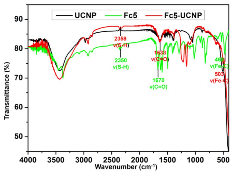
Figure S6. FTIR spectra of UCNP (black line), Fc5 (green line) and Fc5-UCNP (red line).
