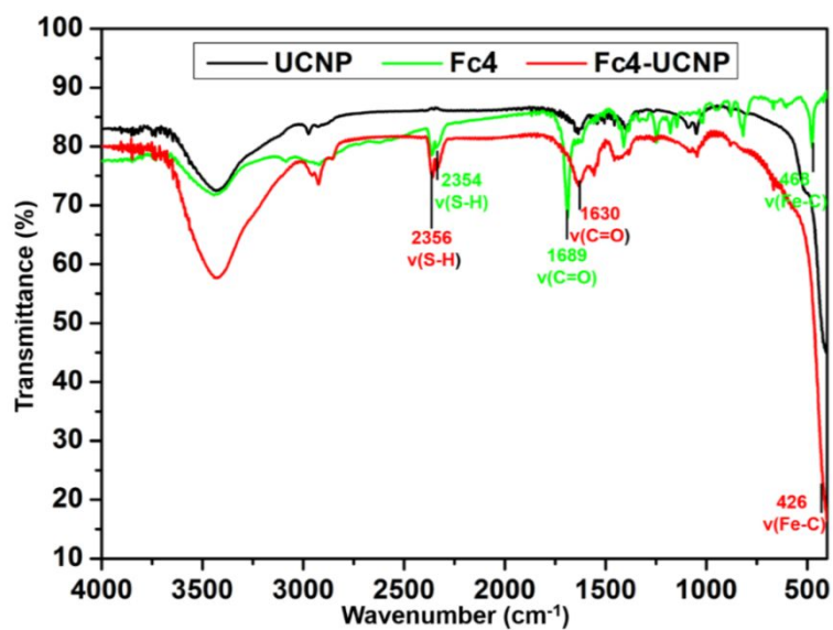
Figure S5. FTIR spectra of UCNP (black line), Fc4 (green line) and Fc4-UCNP (red line).
