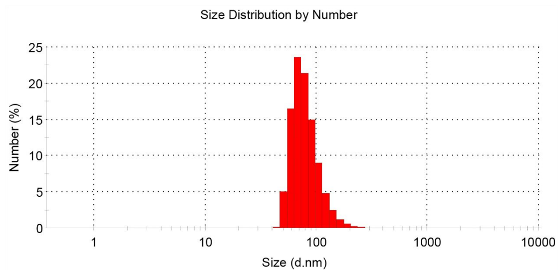
Figure S12. The DLS distribution graph of Fc4 -UCNP-Lipo.
