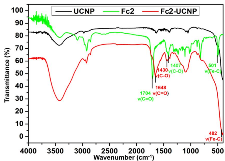
Figure S3. FTIR spectra of UCNP (black line), Fc2 (green line) and Fc2-UCNP (red line).
