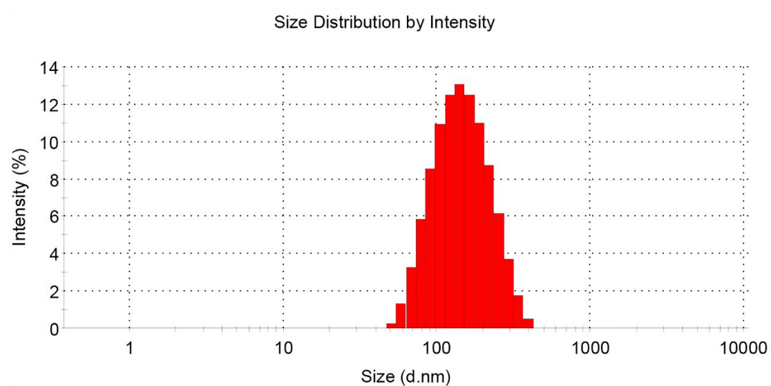
Figure S8. The DLS distribution graph of OA-UCNP-Lipo.
