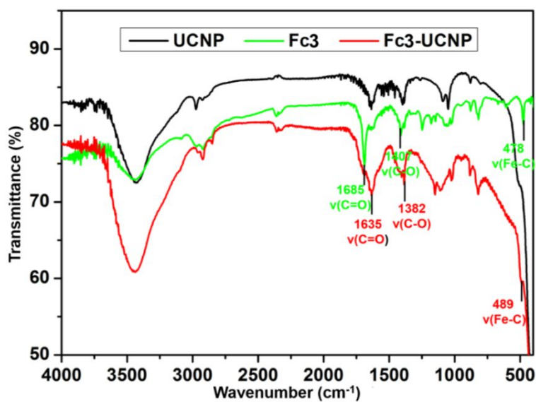
Figure S4. FTIR spectra of UCNP (black line), Fc3 (green line) and Fc3-UCNP (red line).
