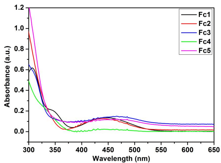
Figure S1. Absorption spectra of Fc1-Fc5 in CH 3 CN.
