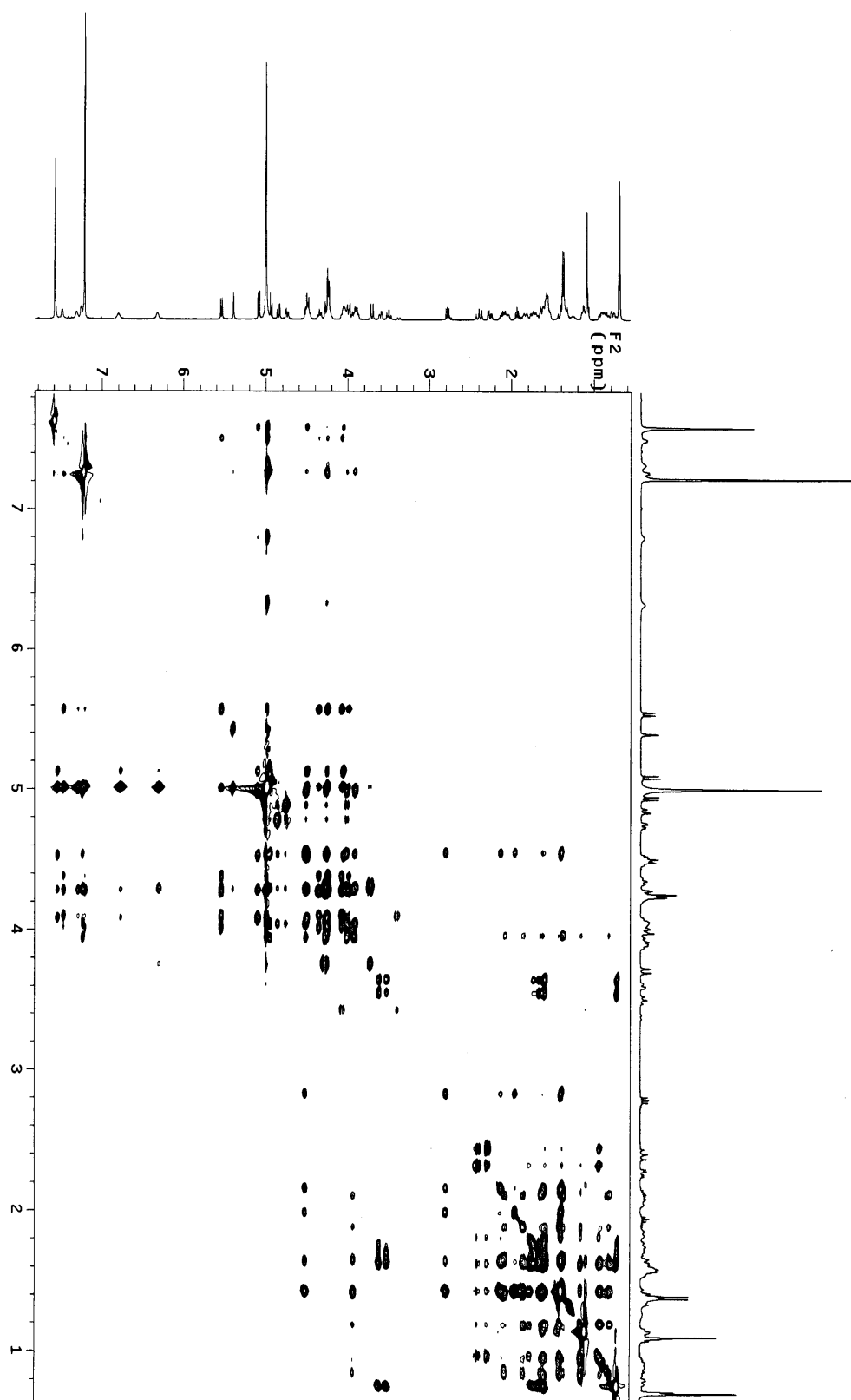
S4. TOCSY spectrum of compound 1 in pyridine- d 5
