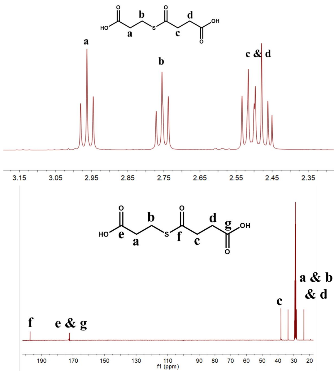
Figure S1 NMR spectrum of CTOA. Top: ^1\text{H} NMR. Bottom: ^{13}\text{C} NMR
