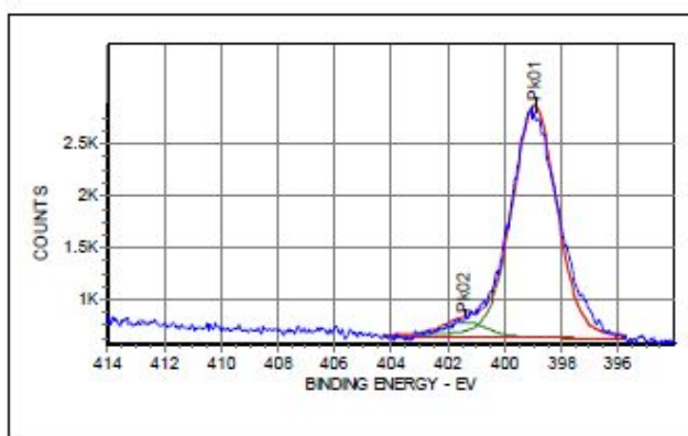
Figure S2. Nitrogen XPS spectrum of antibacterial hyperbranched coating on PDMS
