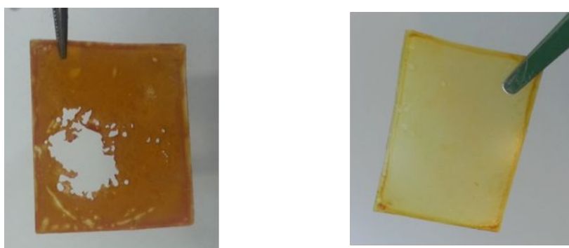
Figure S1. Alkylation with hexyl bromide in the presence of KOH (left) or with a proton sponge ( 1,8-bis(dimethylamino)naphthalene ).
