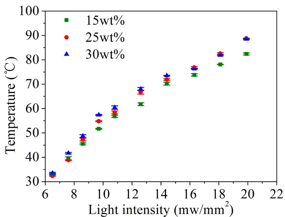
Figure S2. The maximum temperature of actuator varies with concentration and light intensity.
