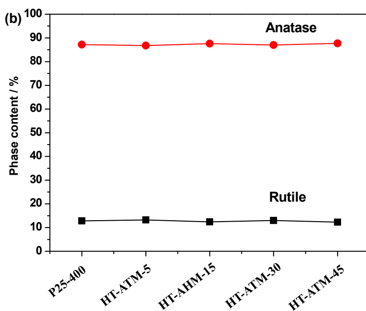
Figure S1 Phase compositions of supported MoS 2 /TiO 2 nanocatalysts with different MoS 2 loadings synthesized by hydrothermal method.
