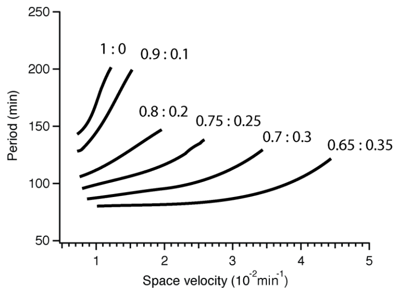
Figure S8. Plot showing the effect of space velocity on the stability and period of oscillation for networks with different values of \chi_{\text{GlySEt}} and \chi_{\text{AlaSEt}} (the ratio of AlaSEt to GlySEt for each simulation are listed above the corresponding trace). Simulations were performed with initial concentrations of [thioester] = 46 mM, [cystamine] = 92 mM, [maleimide] = 10 mM, [acrylamide] = 320 mM.
