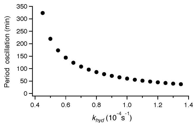
Figure S11. Influence of the value of k_{hyd} on the period of oscillation. The space velocity for each simulation was constant at 1.2 \times 10^{-2} \text{ min}^{-1} and initial concentrations were [\text{Thioester}] = 46 \text{ mM} , [\text{Mal}] = 10 \text{ mM} . These simulations were performed for networks with only one thioester that forms ethanethiol through hydrolysis alone but with different values of k_{hyd} .
