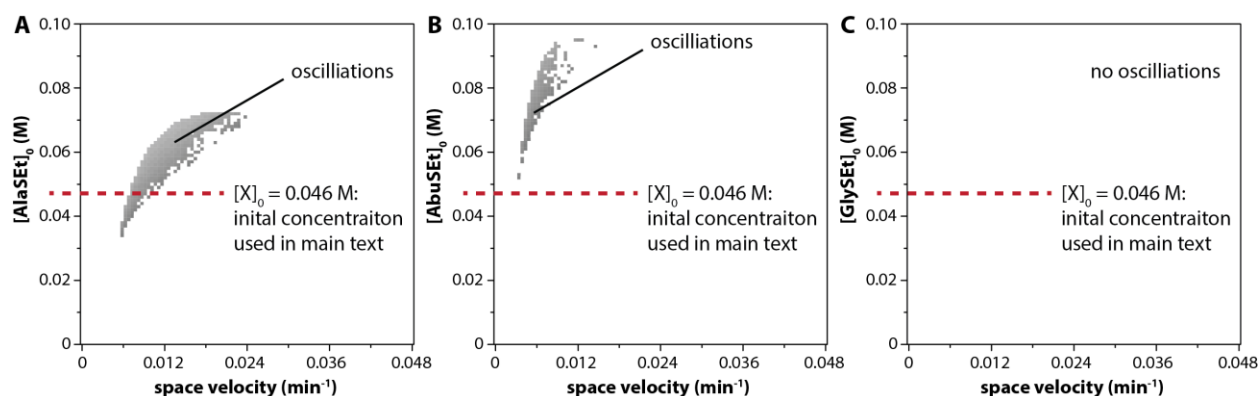
Figure S3. Phase plots showing the relationship between concentration of thioester and space velocity on oscillatory behavior for the network with a single thioester component, (A) AlaSEt, (B) AbuSEt, and (C) GlySEt. The regions that support oscillations are shown in grey, and the red dashed line shows the initial concentration used in experiments. The concentration of other reactants (cystamine, maleimide, and acrylamide) were fixed at 0.092 M, 0.010 M, and 0.320 M, respectively. The phase plots are constructed using independently simulated time series (that are analyzed for the occurrences of oscillatory behavior) using a combination of the space velocity (which is varied from 0 – 0.050 \text{min}^{-1} ) and the initial concentration of the thioesters (which is varied from 0 – 0.10 M). In total, 10,000 simulations were performed for each phase plot.
