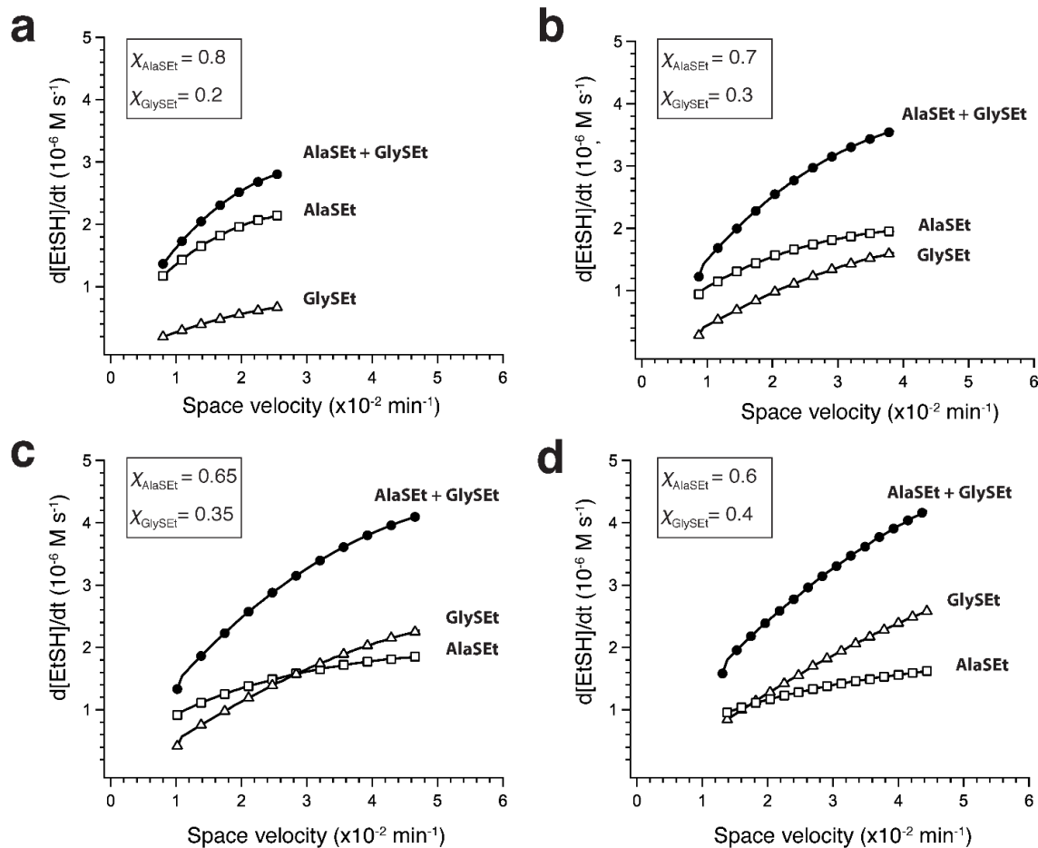
Figure S10. Influence of space velocity on the rate of formation of ethanethiol from aminolysis of GlySEt (open triangles) and hydrolysis of AlaSEt (open squares) together with the summed rate of formation of ethanethiol (filled circles) at the end of the triggering step for networks with (a) \chi_{\text{GlySEt}} = 0.2 and \chi_{\text{AlaSEt}} = 0.8 , (b) \chi_{\text{GlySEt}} = 0.3 and \chi_{\text{AlaSEt}} = 0.7 , (c) \chi_{\text{GlySEt}} = 0.35 and \chi_{\text{AlaSEt}} = 0.65 , and (d) \chi_{\text{GlySEt}} = 0.4 and \chi_{\text{AlaSEt}} = 0.6 .
