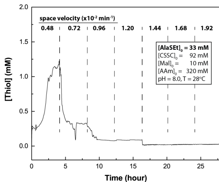
Figure S6. Plot showing the (non-oscillatory) formation of thiol at different space velocities in a reaction network containing AlaSEt alone at an initial concentration of 33 mM ( \chi_{\text{AlaSEt}} = 0.7 ). The space velocity was increased over time with values (in units of 10^{-2} \text{ min}^{-1} ) listed in the plot. Other experimental conditions are reported in the insert.
