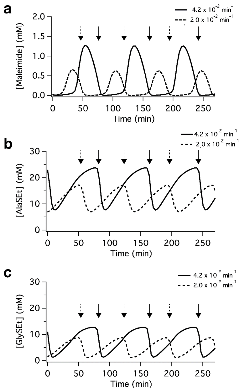
Figure S9. Influence of space velocity on the concentration of (a) maleimide, (b) AlaSEt, and (c) GlySEt in a network that contained a ratio of AlaSEt to GlySEt of 6:4. The simulations were performed at two space velocities, 4.2 \times 10^{-2} \text{ min}^{-1} and 2.0 \times 10^{-2} \text{ min}^{-1} . See list of ordinary differential equations used for modeling above. Arrows indicate time points when the network transitioned to the auto-amplification step, solid lines for the space velocity of 4.2 \times 10^{-2} \text{ min}^{-1} and dashed lines for the space velocity of 2.0 \times 10^{-2} \text{ min}^{-1} .
