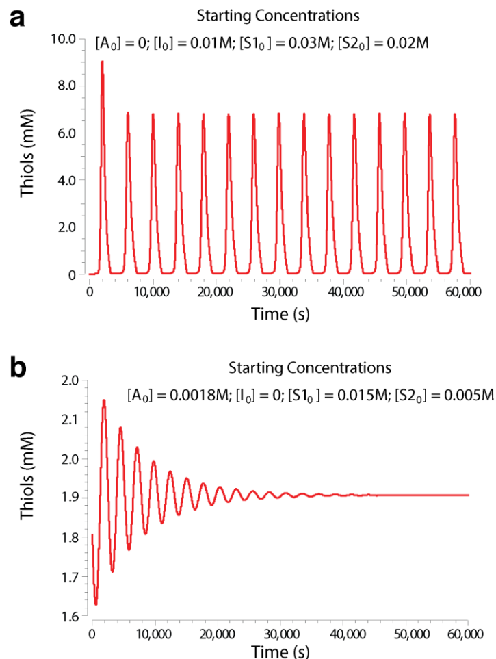
Figure S13. Coexistence of a locally stable steady state and sustained oscillations in the four-variable model of the thiol oscillator with AlaSEt and GlySEt ( \chi_{\text{AlaSEt}} = 0.6 ; \chi_{\text{GlySEt}} = 0.4 ). Both plots ( a and b ) were obtained from the same model ( I_0 = 0.01 \text{ M} , S_{01} = 0.03 \text{ M} , S_{02} = 0.02 \text{ M} , k_0 = 0.0006 \text{ s}^{-1} , k_{11} = 0.25 \text{ s}^{-1}\text{M}^{-1} , k_{12} = 0.8 \text{ s}^{-1}\text{M}^{-1} , k_2 = 300 \text{ s}^{-1}\text{M}^{-1} , k_3 = 0.0055 \text{ s}^{-1} , k_{41} = 8 \cdot 10^{-5} \text{ s}^{-1} , k_{42} = 9 \cdot 10^{-5} \text{ s}^{-1} , k_5 = 0.0306 \text{ s}^{-1}\text{M}^{-1} ) but with different initial conditions. Initial conditions in a are far from steady state values and conditions in b are close to steady state values ( A_{\text{SS}} = 0.00191 \text{ M} , I_{\text{SS}} = 1 \cdot 10^{-5} \text{ M} , S1_{\text{SS}} = 0.0156 \text{ M} , S2_{\text{SS}} = 0.0051 \text{ M} ).
