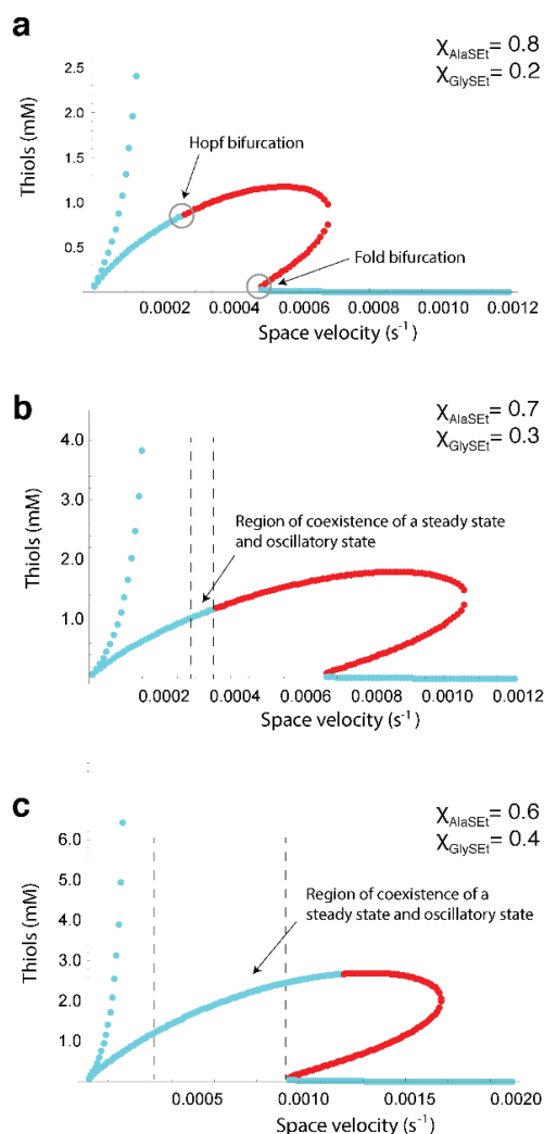
Figure S12. Results from linear stability analysis of mixtures of AlaSEt and GlySEt. Blue points represent stable steady states and red points represent unstable steady states. Mole fraction of AlaSEt to GlySEt examined were (a) 0.8:0.2, (b) 0.7:0.3, and (c) 0.6:0.4. We determined the area of coexistence of a steady state and sustained oscillations through numerical integration of the equations of the four-variable model. Specifically, we integrated the equations with initial conditions [A_0] = 0 ; [I_0] = 0.01 \text{ M} ; [S1_0] = S_{01} ; [S2_0] = S_{02} and considered that a region of the parameter space contains a stable orbit if we observe sustained oscillations with these initial conditions for 500 hours. For an example of coexistence of a locally stable steady state and sustained oscillations see Figure S12.
