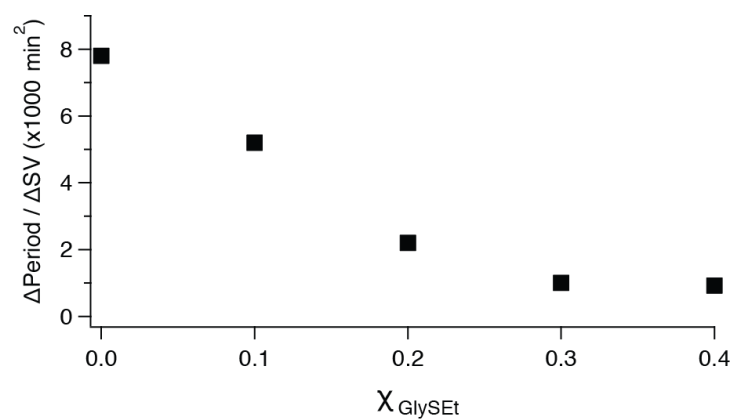
Figure S7. Plot of the change in period as a function of the change in space velocity from the linear fits in Figure 4c. The plot shows the influence of the mole fraction ( \chi_{\text{GlySEt}} ) on the sensitivity of the frequency of oscillation to change in space velocity.
