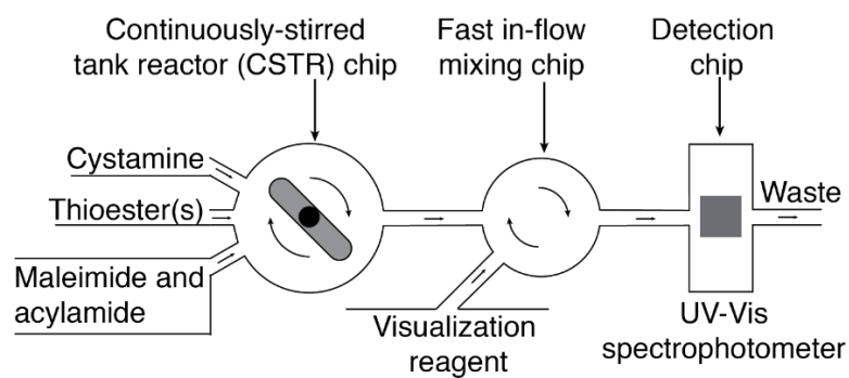
Figure S1. Schematic representation of the continuous stirred-tank reactor (CSTR). In this apparatus, syringe pumps feed reactants to the inlet ports of the CSTR. For continuous sampling, a tube connected to the outlet port of the CSTR takes the effluent (products and reactants) to a fast in-flow mixing detection chip.
