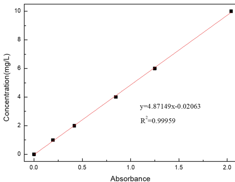
Figure S2. Concentration-adsorption standard curve of RhB solution
