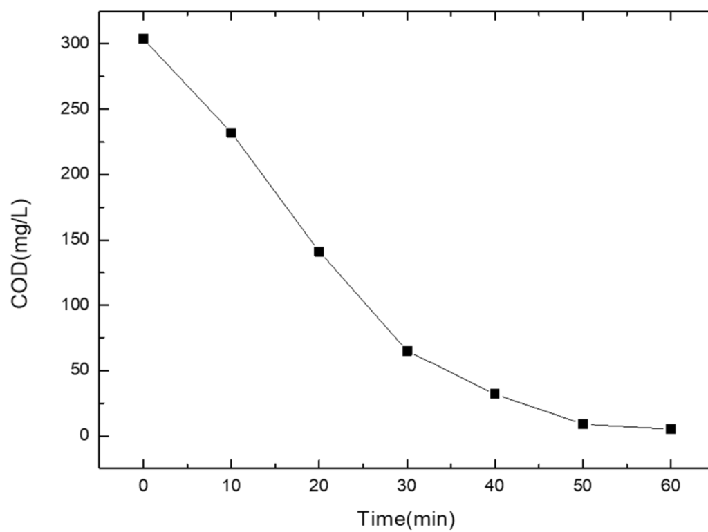
Figure S3. Chemical oxygen demand (COD) for RhB solution in the presence of
