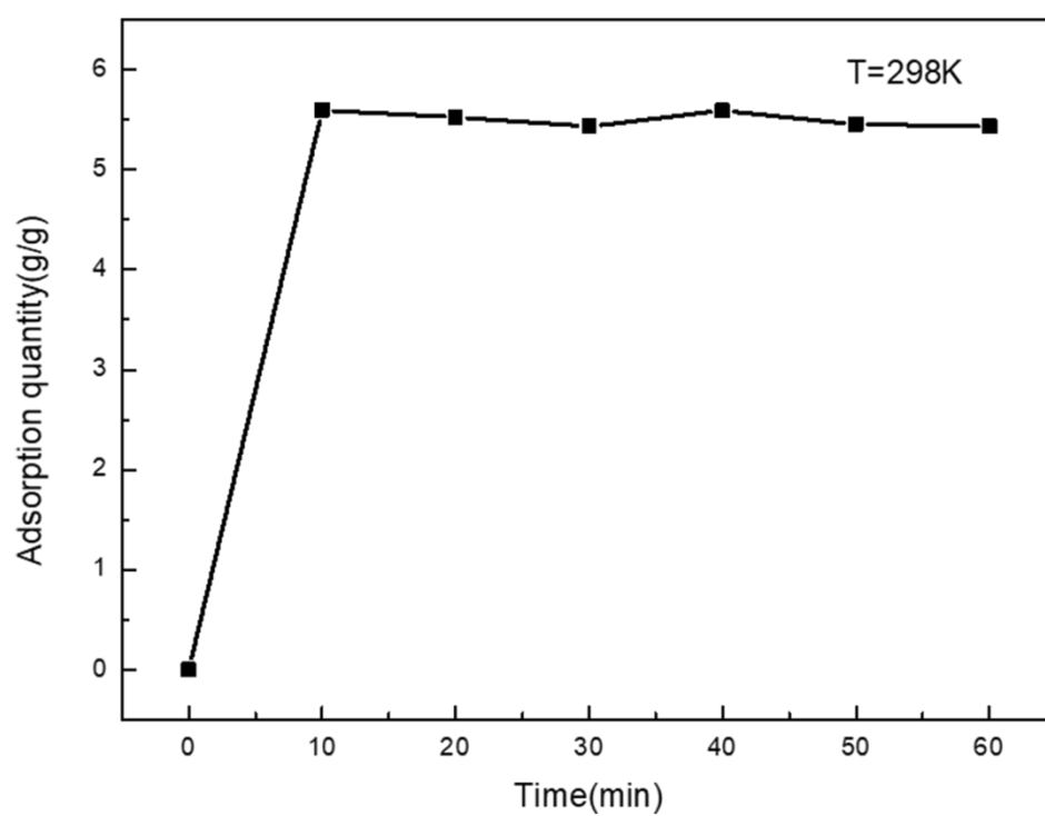
Figure S1. Adsorption isothermal curve of g-C 3 N 4 /MWCNTs-2 for the RhB solution of 10 mg L -1 at 298 K.
