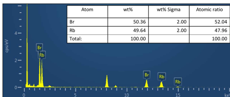
Figure S1. The energy-dispersive X-ray spectroscopy result of the hollow RbBr nanocubes.
