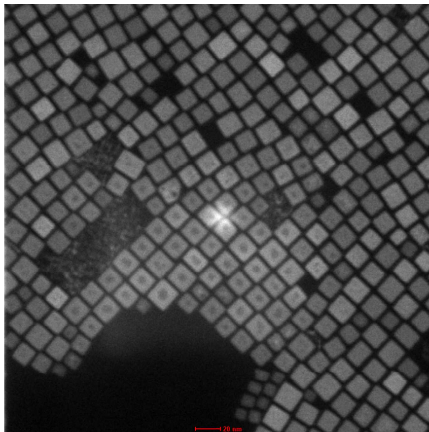
Figure S2. The HAADF image of the RbBr nanocubes showing voids only appeared in the area with focused e-beam.
