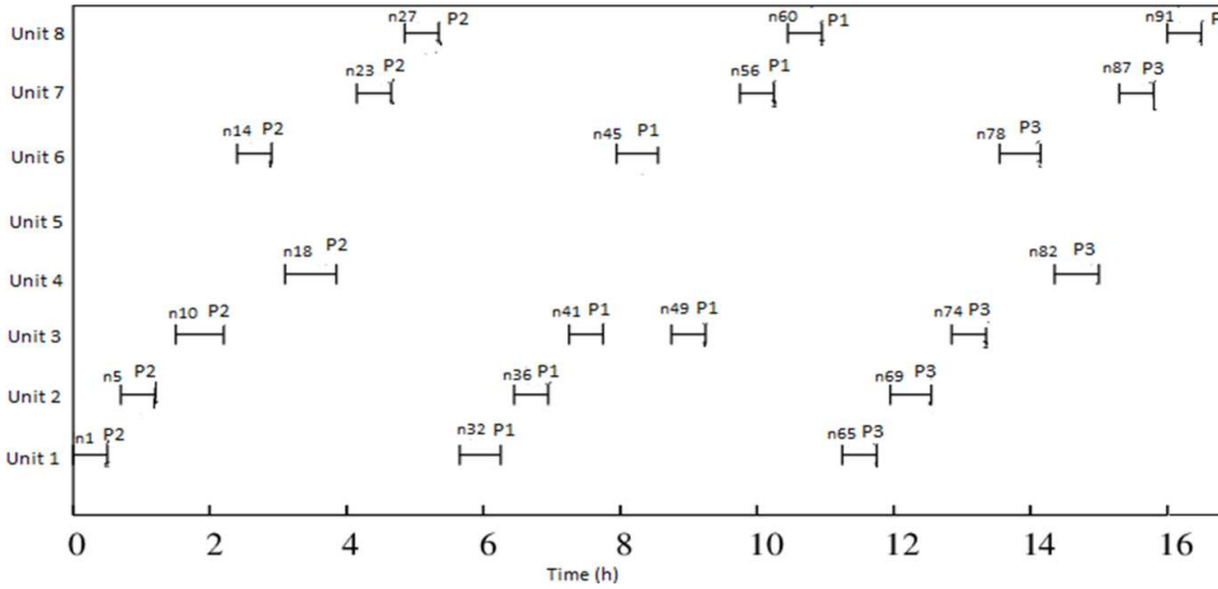
Figure S2. Gantt chart for single vessel case in circular layout (example 1)
