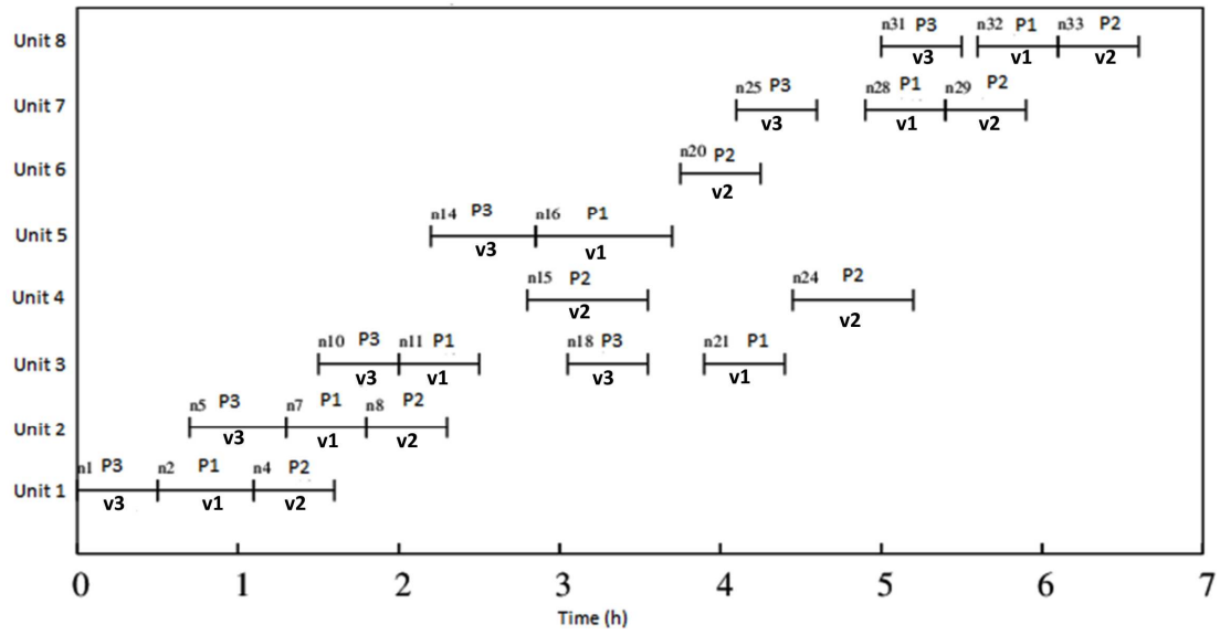
Figure S3. Gantt chart for three vessel case in linear layout (example 1)
