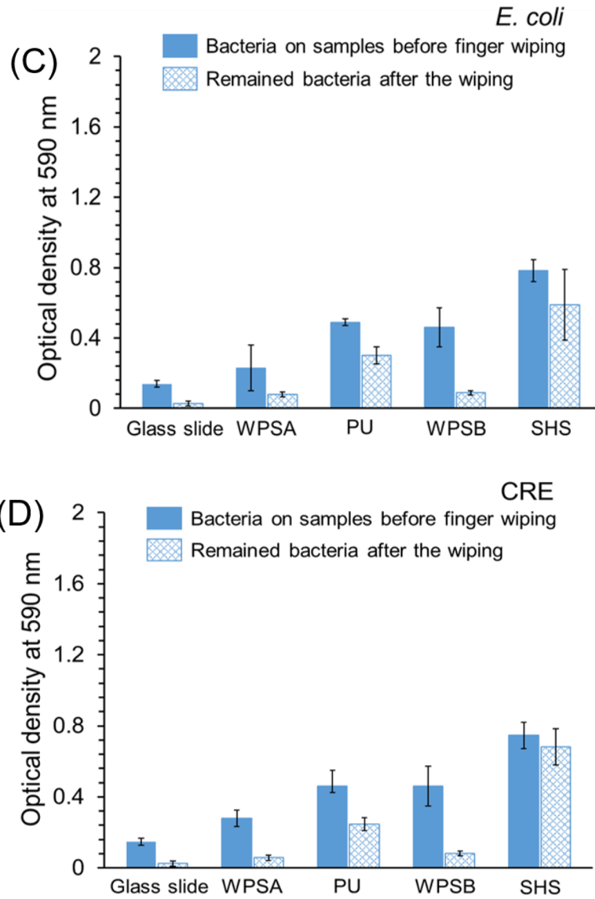
Figure S11. Comparison of the quantity of bacteria on the materials before and after finger wiping: (a) S. aureus , (b) MRSA, (c) E. coli , and (d) CRE.
