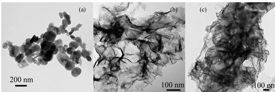
Figure S1. Typical TEM images of the three BN support, BN c (a), BN s (b) and BN p (c)
