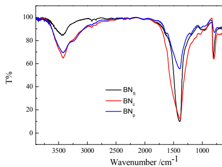
Figure S2. Typical FT-IR spectra of the three BN supports.
