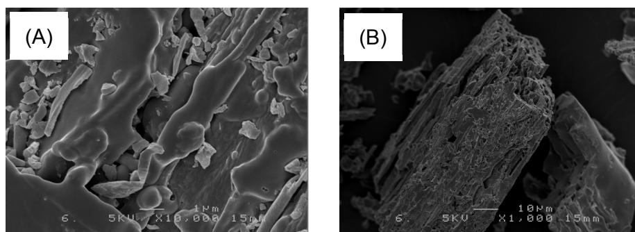
Figure S1. SEM images of the recycled adsorbents (Entry 9 in Table 1) prepared by thermal treatment of at 350 °C for 1 h under oxygen atmosphere with 10,000 (A) and 1,000 (B) magnifications.
